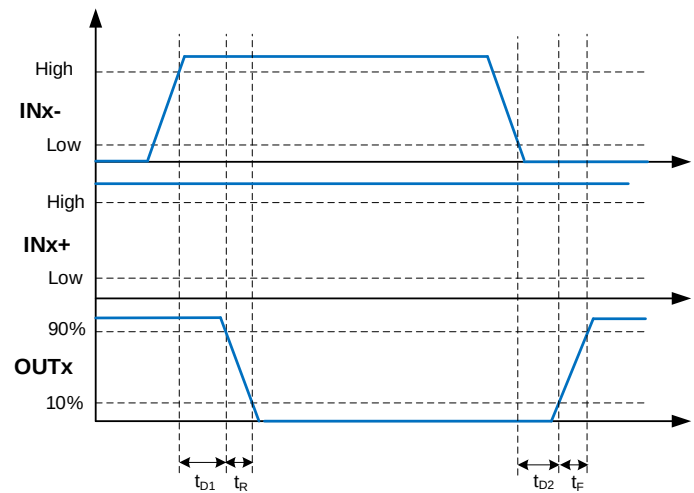
Figure 4. Inverting Input Driver Operation
