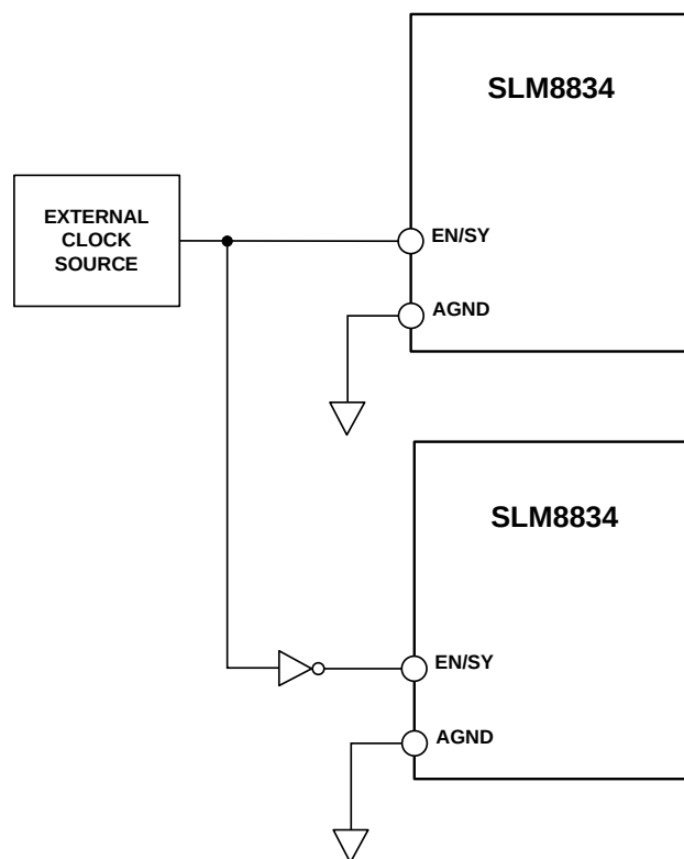
Figure 14. Multiple SLM8834 Devices Driven from a Master Clock
